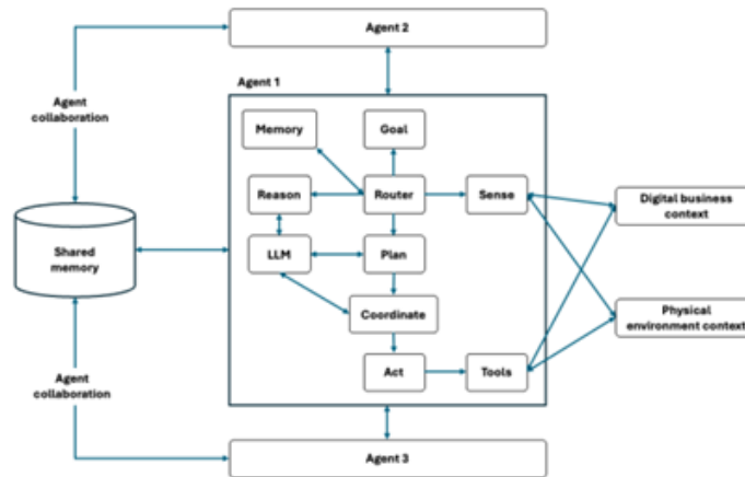
Figure 2.7: Agentic AI anatomy [23]
